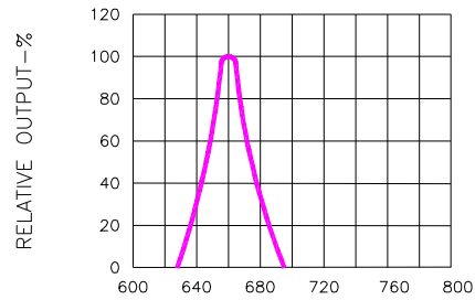
Fig.2 SPECTRAL RESPONSE
