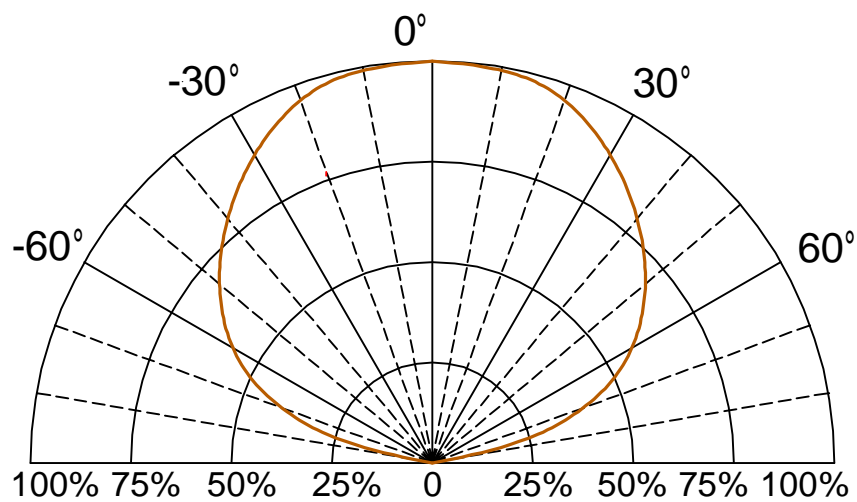
Fig.6 Directivity Radiation
