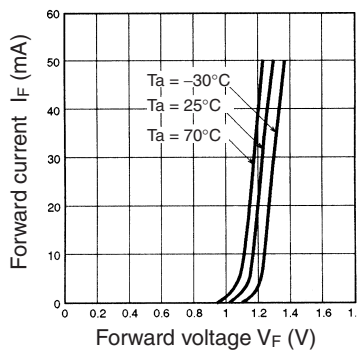
Forward Current vs. Forward Voltage Characteristics (Typical)
