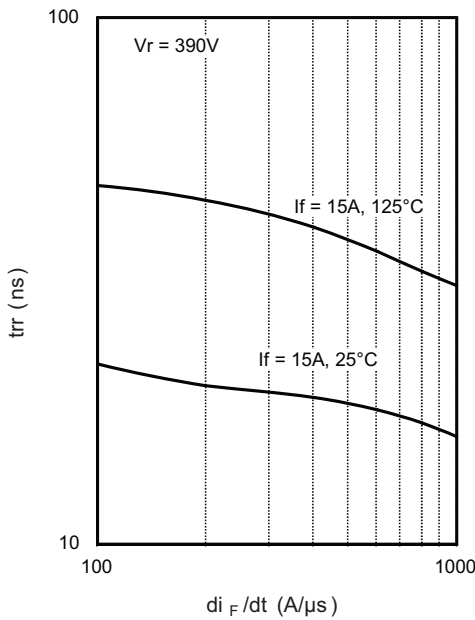
Fig. 7 - Typical Reverse Recovery Time vs. di F /dt
