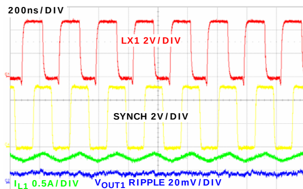
FIGURE 32. CH1 STEADY STATE OPERATION AT FULL LOAD (PFM) WITH FREQUENCY = 4MHz
