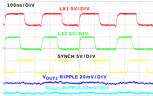
FIGURE 36. CH1 AND CH2 STEADY STATE OPERATION AT FULL LOAD (PFM) WITH FREQUENCY = 4MHz
