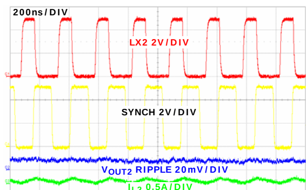
FIGURE 33. CH2 STEADY STATE OPERATION AT NO LOAD (PFM) WITH FREQUENCY = 4MHz
