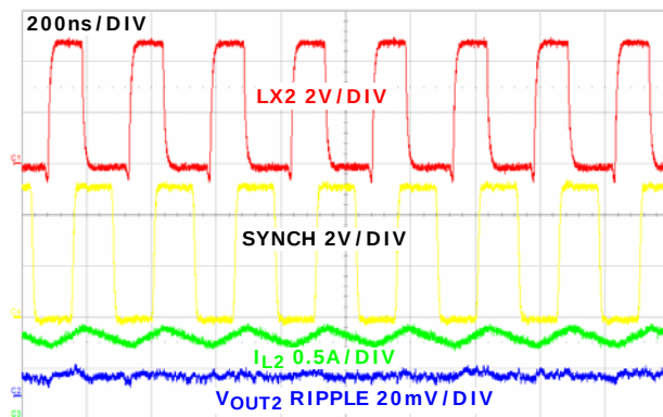
FIGURE 34. CH2 STEADY STATE OPERATION AT FULL LOAD (PFM) WITH FREQUENCY = 4MHz
