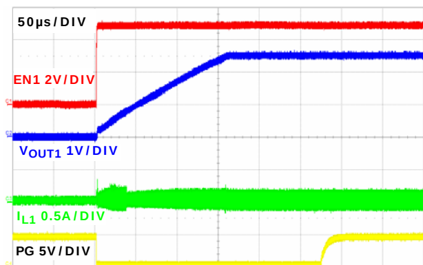
FIGURE 23. SOFT-START WITH NO LOAD CHANNEL 1 (PWM)
