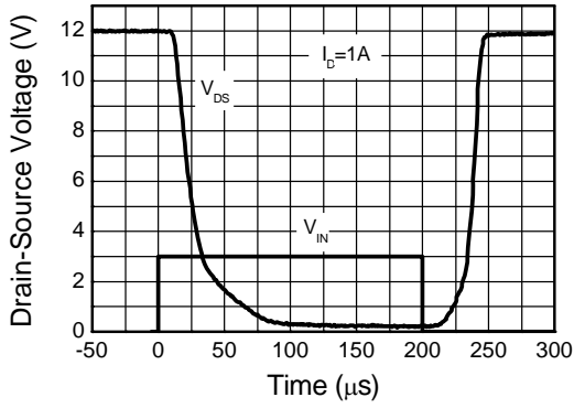
Switching Speed
