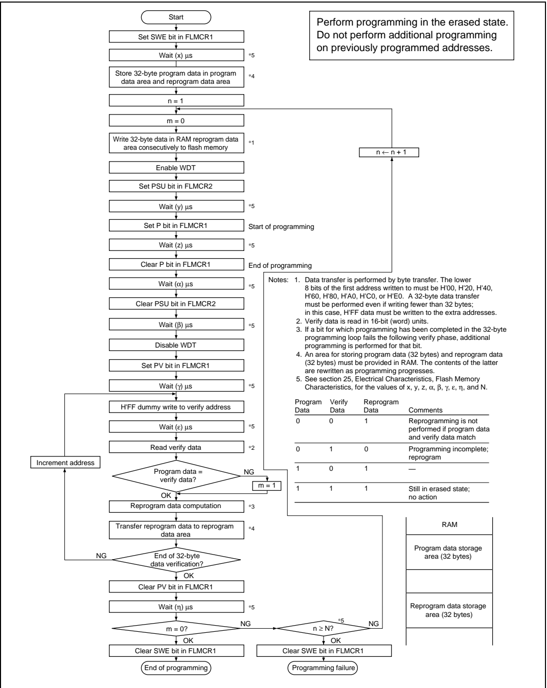
Figure 21.12 Program/Program-Verify Flowchart
