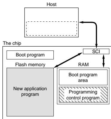
Figure 22.4 Boot Mode
