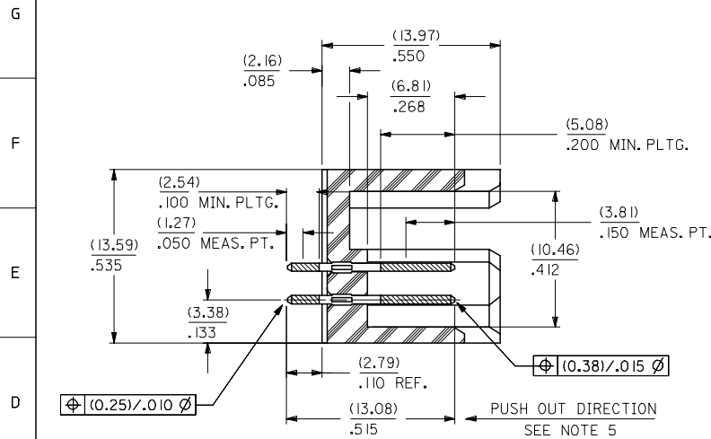
SECTION W-W
