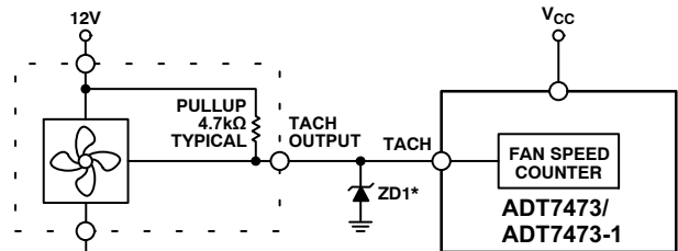
Figure 41. Fan with TACH Pullup to Voltage > 3.6 V Clamped with Zener Diode
