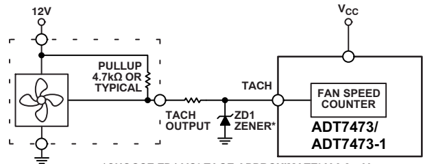
Figure 42. Fan with Strong TACH Pullup to > V CC or Totem-Pole Output, Clamped with Zener and Resistor
