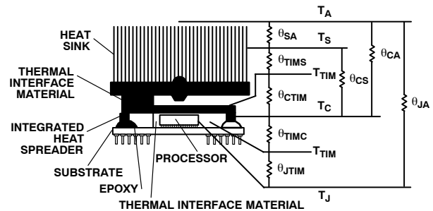
Figure 65. Thermal Model
