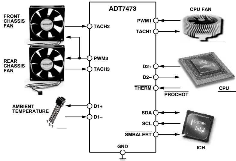
Figure 12. ADT7473 Configuration
