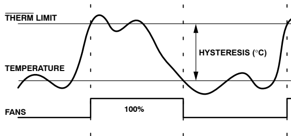
Figure 28. \overline{\text{THERM}} Temperature Limit Operation
