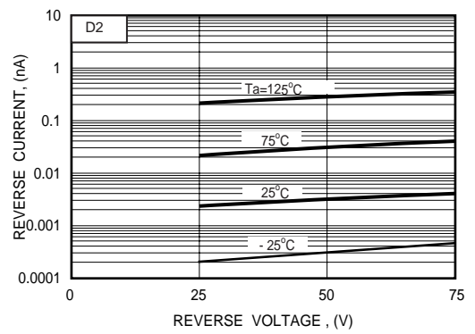
FIG. 4 - REVERSE CHARACTERISTICS
