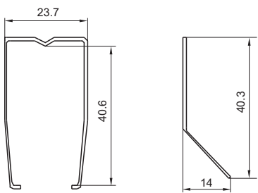
18FF-H5 (Steel retainer)
