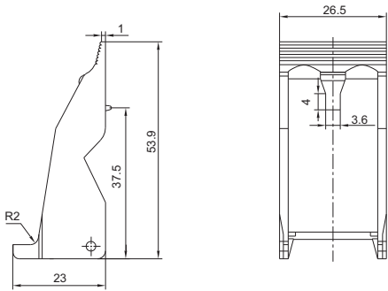
18FF-H4 (Plastic retainer)
