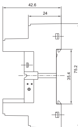
Outline Dimensions
