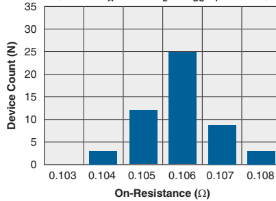
Typical On-Resistance Distribution (N=50, T_A=25^\circ\text{C} , I_L=1\text{A}_{\text{DC}} , I_F=10\text{mA} )
