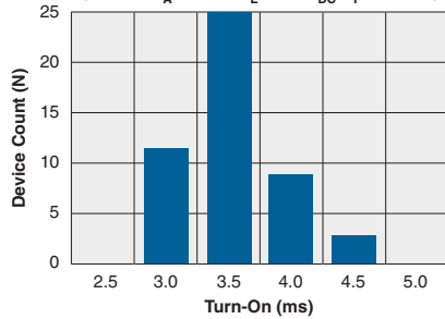
Typical Turn-On Time (N=50, T_A=25^\circ\text{C} , I_L=5\text{mA}_{\text{DC}} , I_F=10\text{mA} )
