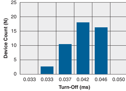
Typical Turn-Off Time (N=50, T_A=25^\circ\text{C} , I_L=5\text{mA}_{\text{DC}} , I_F=10\text{mA} )
