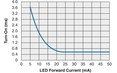
Typical Turn-On vs. LED Forward Current ( I_L=100\text{mA}_{\text{DC}} )
