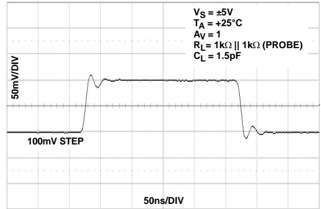
FIGURE 28. SMALL SIGNAL TRANSIENT RESPONSE
