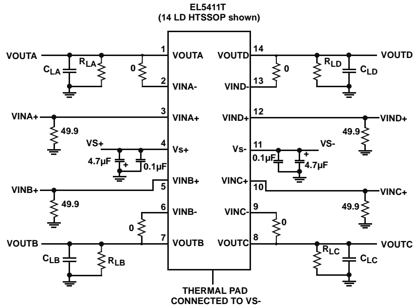
FIGURE 29. BASIC TEST CIRCUIT
