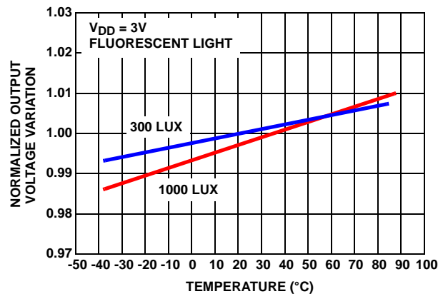
FIGURE 12. NORMALIZED OUTPUT VOLTAGE vs TEMPERATURE
