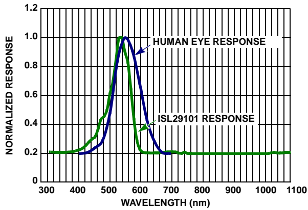
FIGURE 3. SPECTRAL RESPONSE
