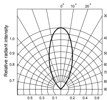
Fig.6 Radiation diagram
