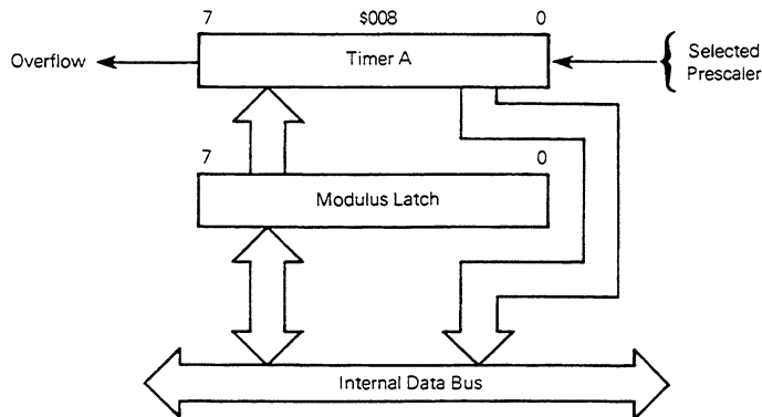
Figure 3-2. Timer A
