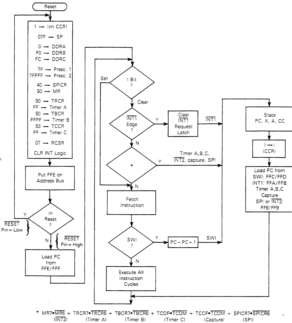
Figure A-4. Reset and Interrupt Processing Operation
