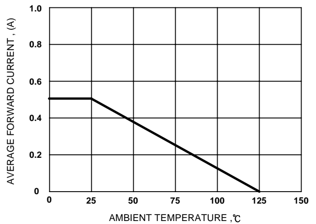
Figure 4. Forward Current Derating Curve
