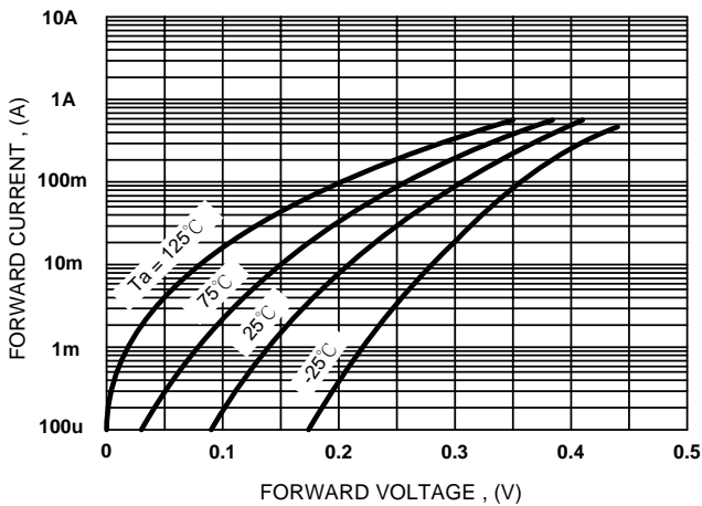
Figure 1. Forward Characteristics
