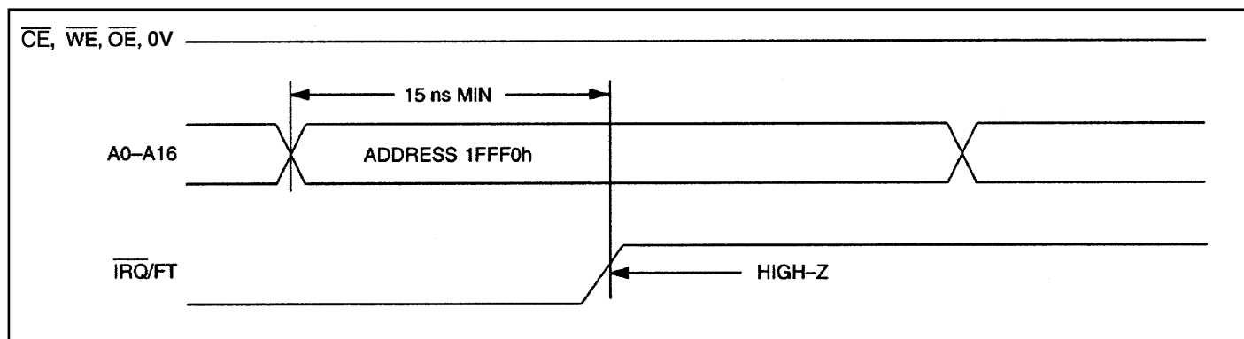
Figure 2. Clearing \overline{\text{IRQ}}/\text{FT} Waveforms
