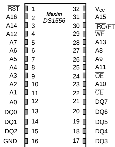
Encapsulated DIP
