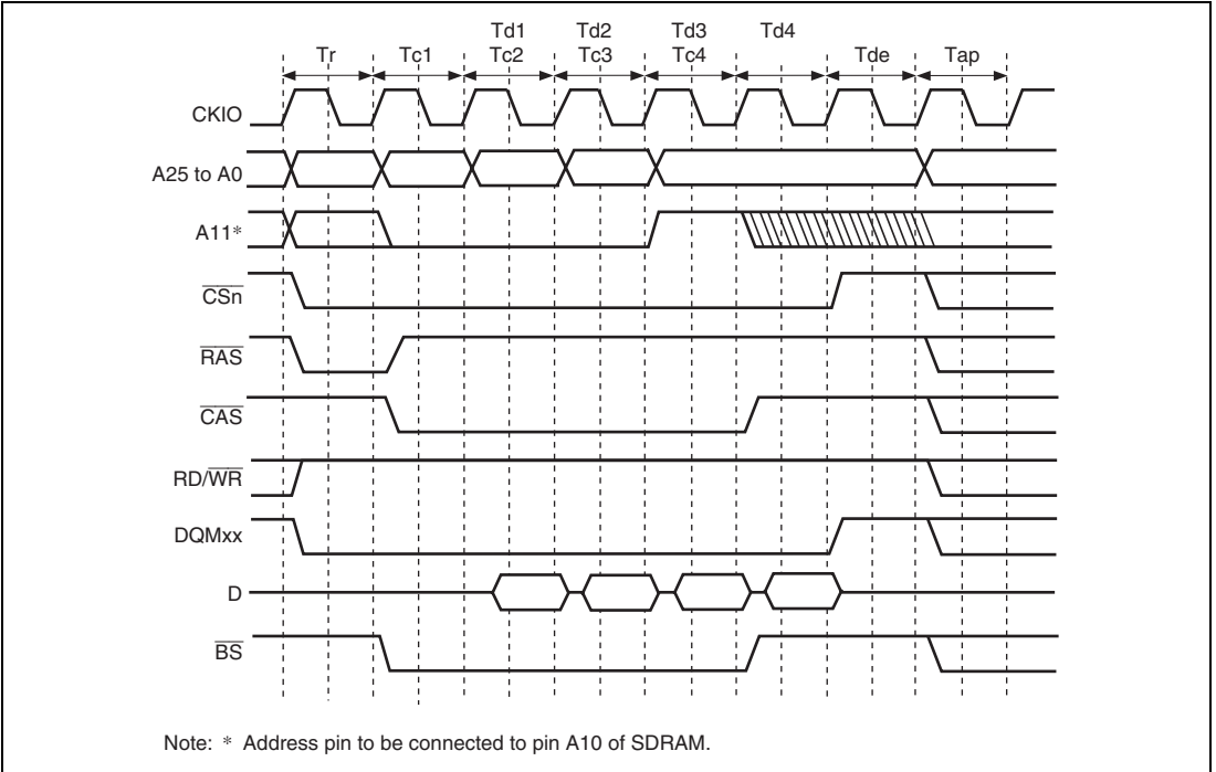
Figure 7.14 Burst Read Basic Timing (Auto Precharge)
