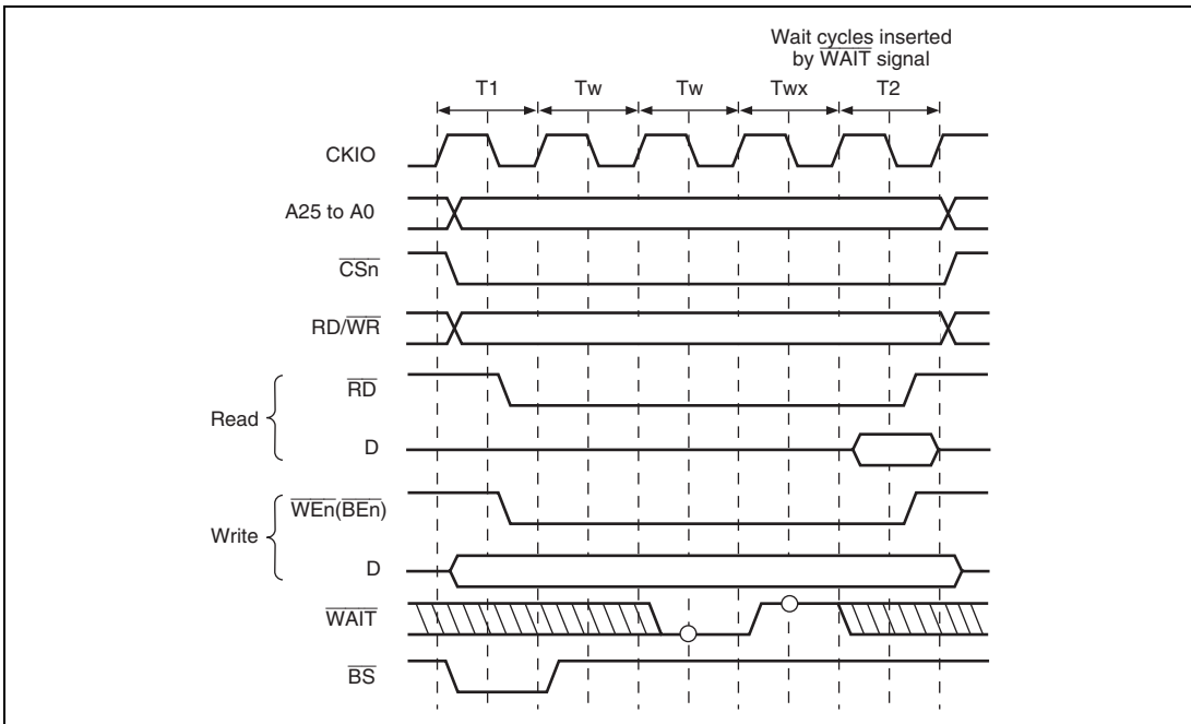
Figure 7.10 Wait Cycle Timing for Normal Space Access (Wait cycle Insertion using \overline{WAIT} )
