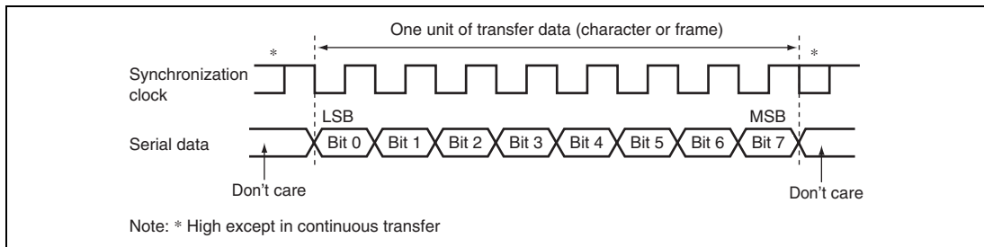
Figure 15.11 Data Format in Synchronous Communication
