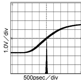
Fig.51 33.9MHz Period-Jitter VDD=3.3V, at CL=15pF
