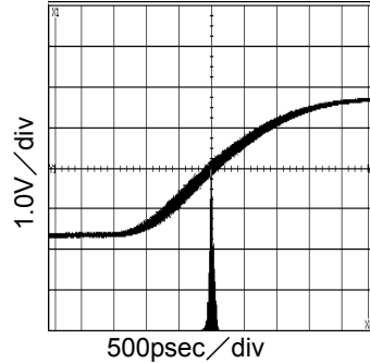
Fig.48 27MHz Period-Jitter VDD=3.3V, at CL=15pF
