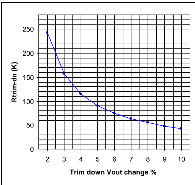
Fig 6 Trim Down Resistance for reference chart
