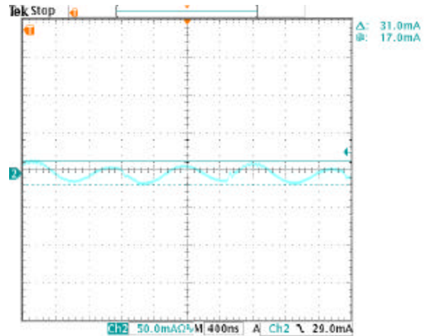
Figure 27. Input reflected ripple current \dot{I}_s waveform With 10uH input inductor. At V_{in}=48v , I_{out}=25A , 50ma/Div ( current probe with 50mv/div )
