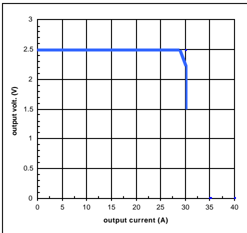
Figure 19. Output voltage vs. output current limit point and the unit shutdown point. Input voltage has almost no effect on current limit point.
