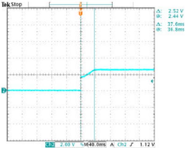
Figure 17. Output voltage over shoot and rise time at Vin=48v, Iout = 0A; with 100uF output capacitance load, and On/Off pin enabled to turn on the unit.
