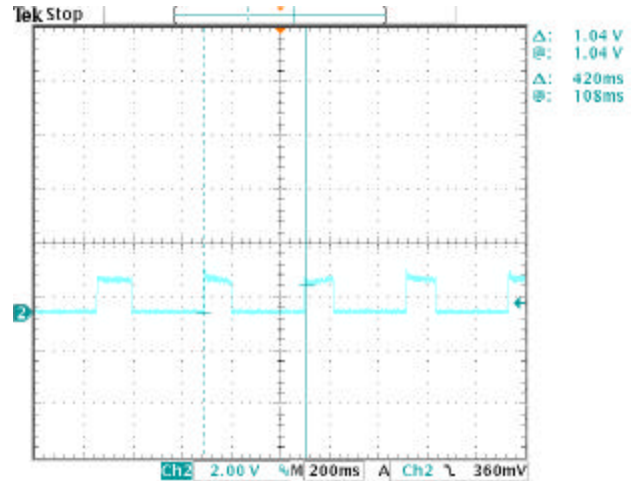
Figure 20. Output waveform under short circuit protection condition. Under 10mΩ short circuit during restart at 48Vin.
