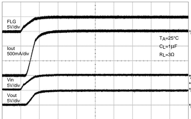
Power On
