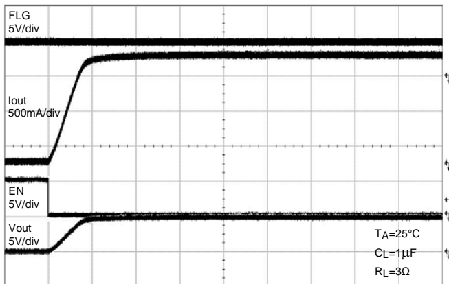
Device Enabled
