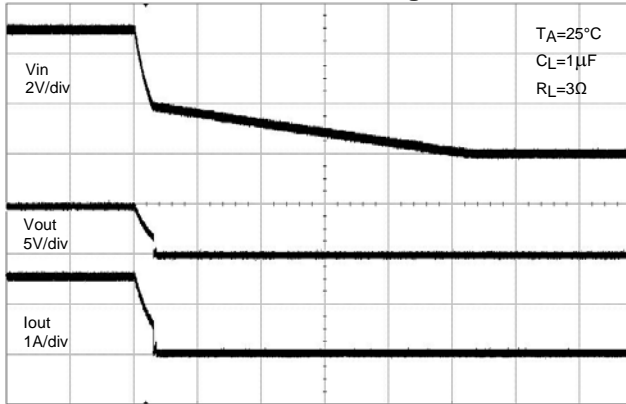
UVLO Decreasing
