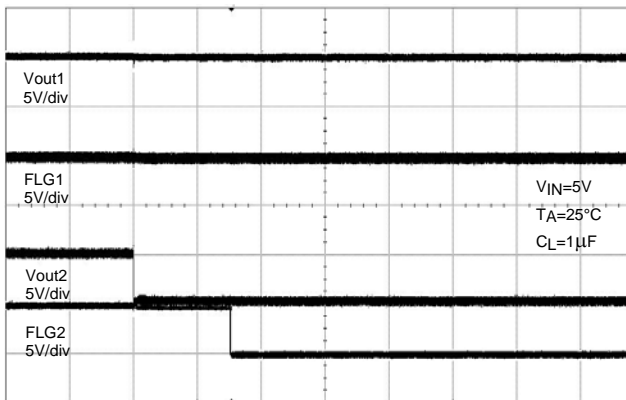
Channel 2 Enabled and Shorted with Channel 1 Enabled
