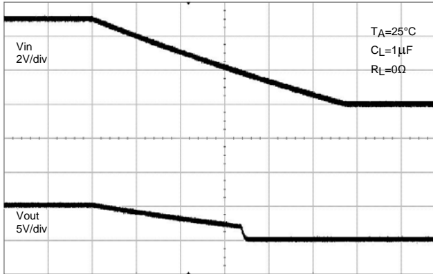
UVLO Decreasing (No Load)
