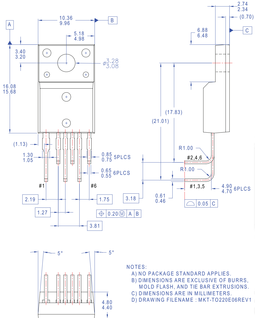
Figure 40. 6-Lead, TO-220 Package (L-Forming)
