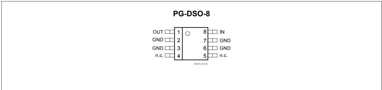
Figure 2 Pin Configuration
