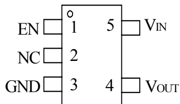
SOT23-5(B) T6328A-XXBXG
