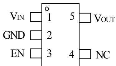
SOT23-5(A) T6328A-XXAXG
