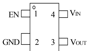
SC-82(A) T6328A-XXAUG
