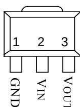
SOT-89(A) T6328A-XXDXG
