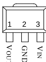
SOT-89(B) T6328A-XXEXG
