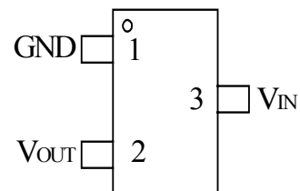
SOT23-3(A) T6328A-XXCXG
