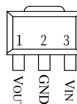
SOT-223(A) T6328A-XXFXG
