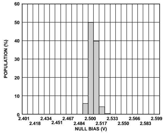
Figure 7. Null Bias at 25°C
