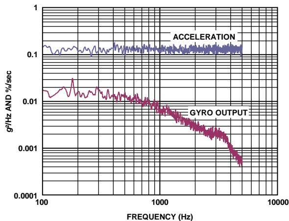
Figure 15. Typical Response to 25 g RMS Random Vibration, 50 Hz to 5 kHz (Sensor Bandwidth = 1 kHz)
