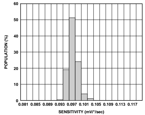
Figure 8. Sensitivity at 25°C
