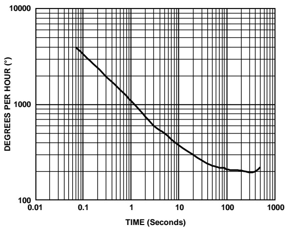
Figure 6. Typical Root Allan Deviation at 25°C vs. Averaging Time
