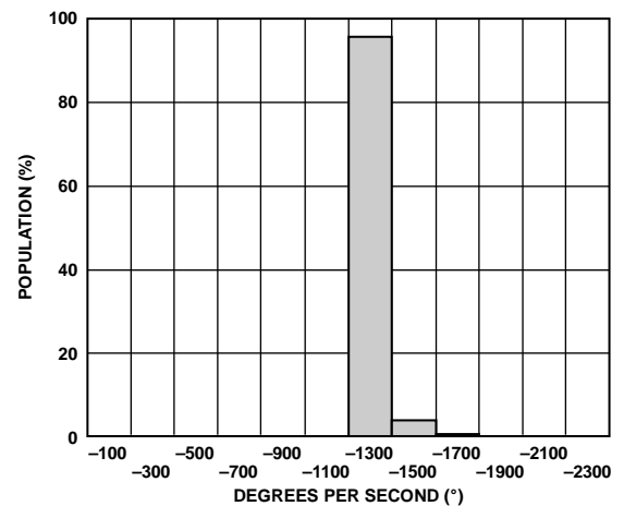
Figure 9. ST1 Output Change at 25°C ( V_{RATIO} = 5 V)
