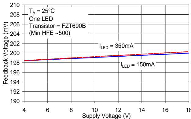
Bipolar transistor driving
