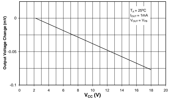
Line regulation
