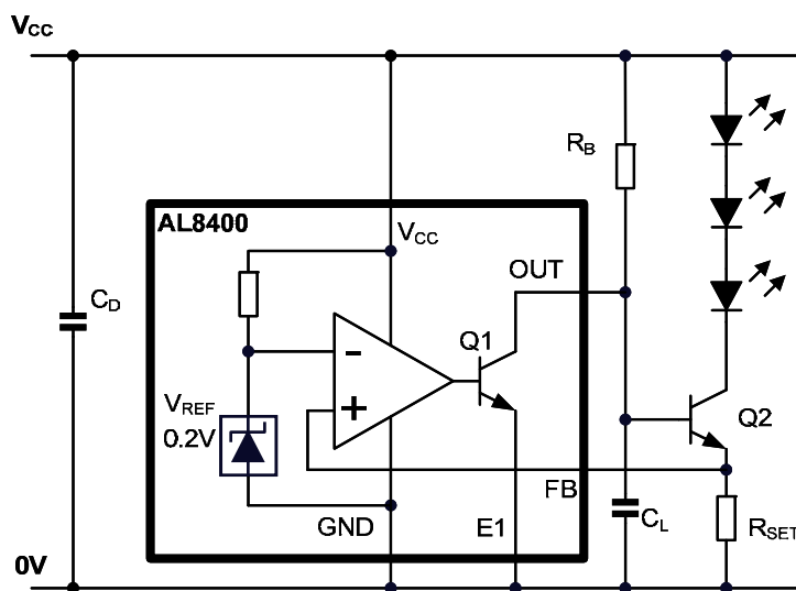
Figure 2. Application Circuit Using Bipolar Transistor
