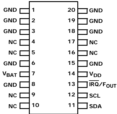
ISL12022MR5421 (20 LD SOIC) TOP VIEW
