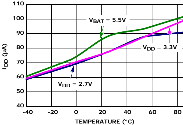
FIGURE 10. I DD WITH TSE = 1 vs TEMPERATURE
