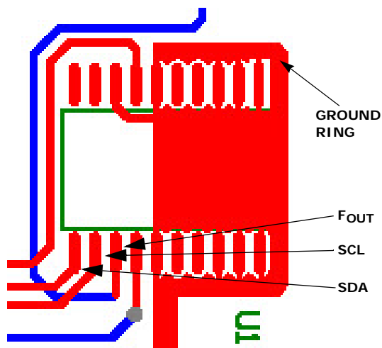
FIGURE 21. SUGGESTED LAYOUT FOR THE ISL12022MR5421
