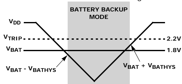
FIGURE 12. BATTERY SWITCHOVER WHEN V_{BAT} < V_{TRIP}
