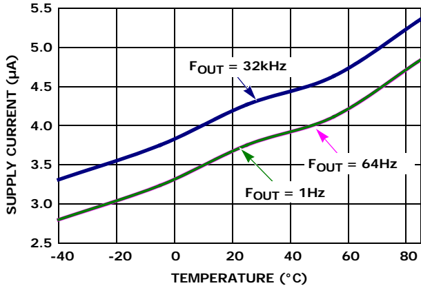
FIGURE 8. I DD vs TEMPERATURE, 3 DIFFERENT F OUT
