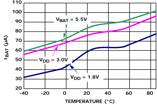
FIGURE 9. I BAT WITH TSE = 1, BTSE = 1 vs TEMPERATURE
