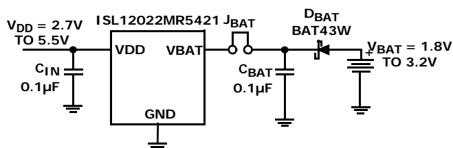
FIGURE 19. SUGGESTED BATTERY BACKUP CIRCUIT
