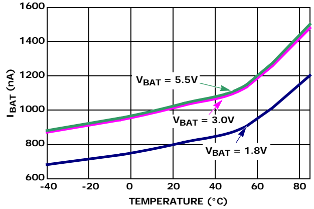
FIGURE 3. I_{BAT} vs TEMPERATURE ( V_{DD} = 0V )
