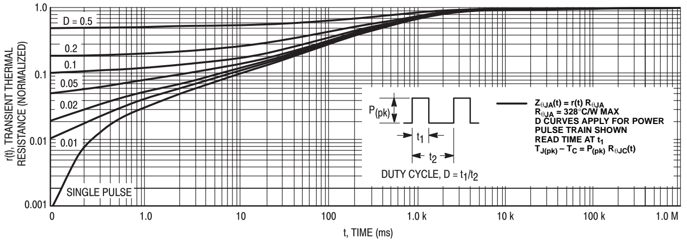
Figure 25. Thermal Response
