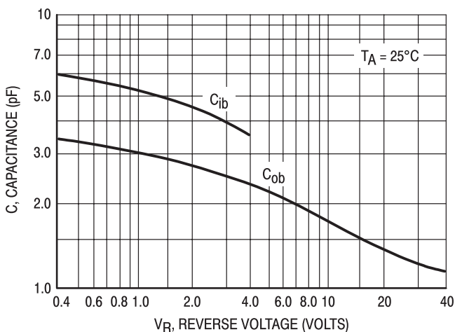
Figure 17. Capacitances
