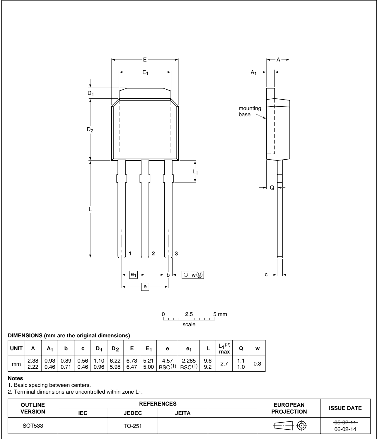
Fig 14. Package outline SOT533 (IPAK)
