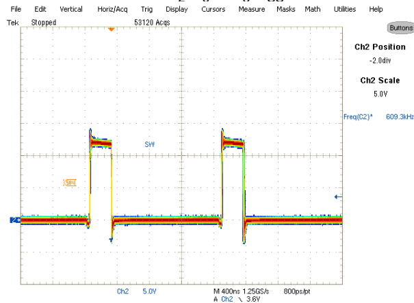
Fig. 11: Inductor node at 12A load Ch 2 :LX
