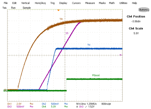
Fig. 8: Start up at 12A Load, Ch 1 :V in , Ch 2 :V o , Ch 3 :V ss , Ch 4 :V PGGood
