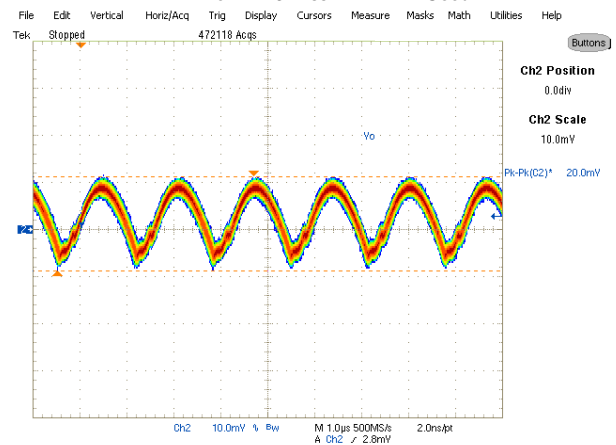
Fig. 10: Output Voltage Ripple, 12A load Ch 2 :V out
