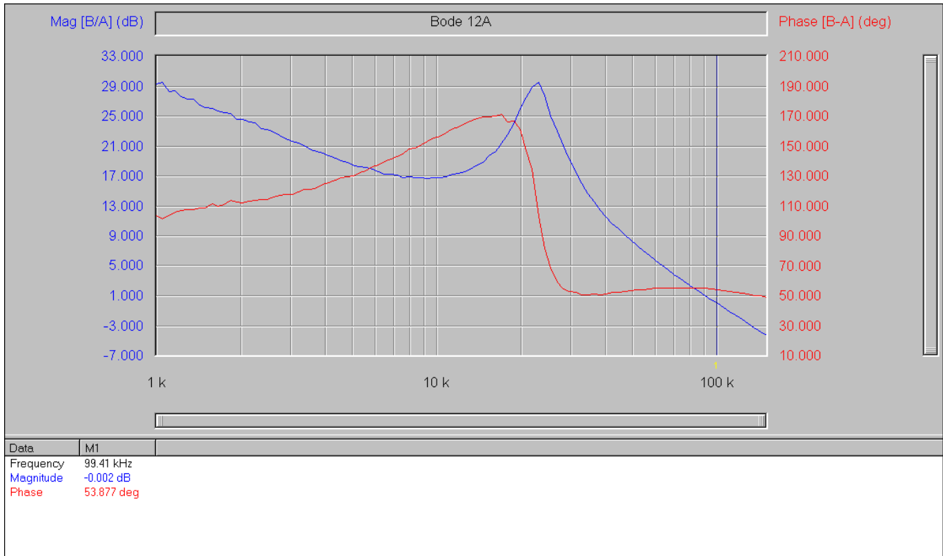
Fig. 14: Bode Plot at 12A load shows a bandwidth of 99kHz and phase margin of 54 degrees
