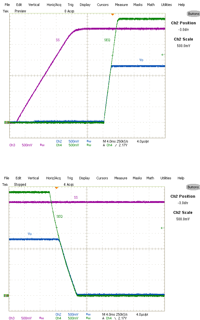
Fig. 18: Simultaneous Tracking a 3.3V input at power-up and shut-down Ch2: SS (1.8V) Ch3:Vo Ch4: SEQ
