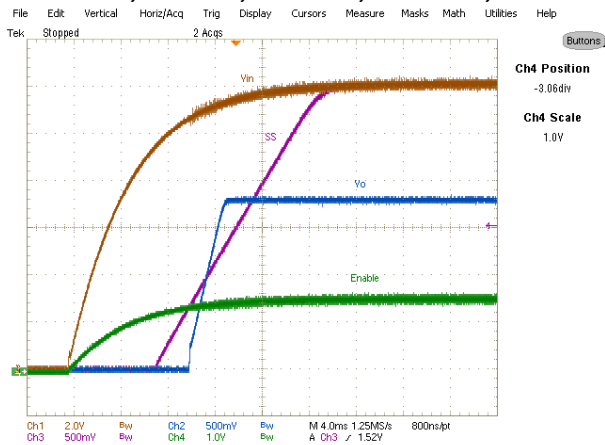
Fig. 7: Start up at 12A Load Ch 1 :V in , Ch 2 :V o , Ch 3 :V ss , Ch 4 :Enable
