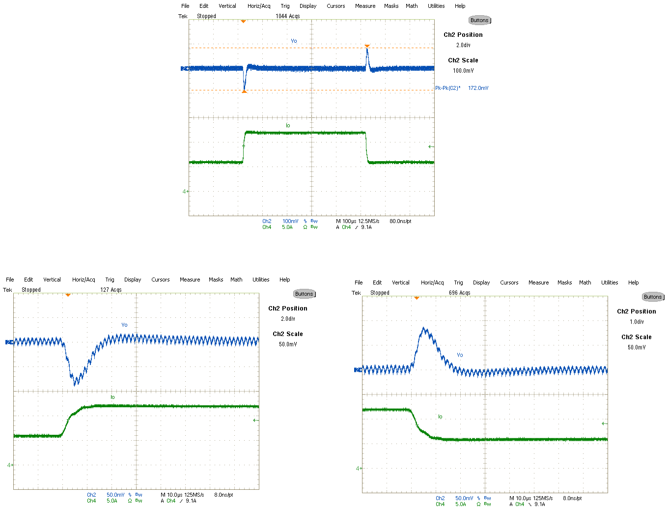
Fig. 13: Transient Response, 6A to 12A step 2.5A/ \mu s Ch 2 :V out , Ch 4 :I out
