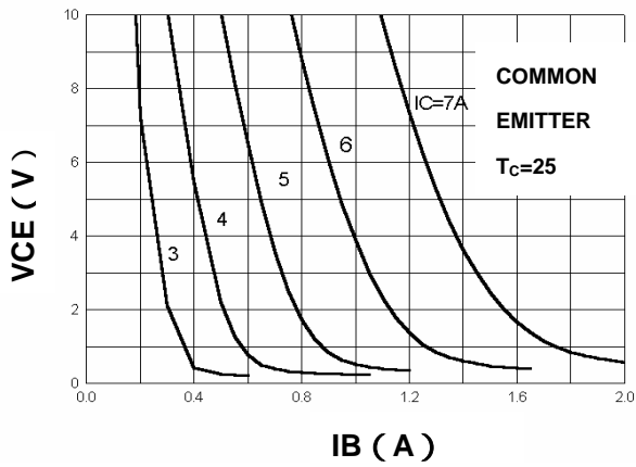
VCE - IB
