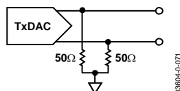
Figure 2. Diagram Showing Termination of 100 Ω Differential Load for Some TxDAC Measurements
