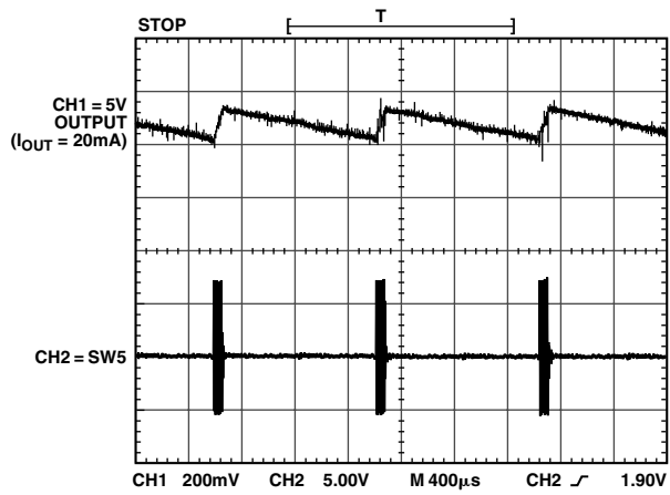
TPC 14. Power-Saving Mode, Waveforms
