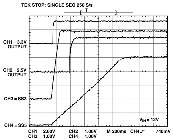
TPC 12. Soft-Start Sequencing
