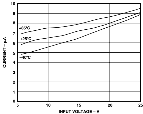
TPC 8. Input Shutdown Current vs. Input Voltage
