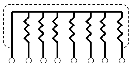
Fig. 1: BUSSED/COMMON CIRCUIT
