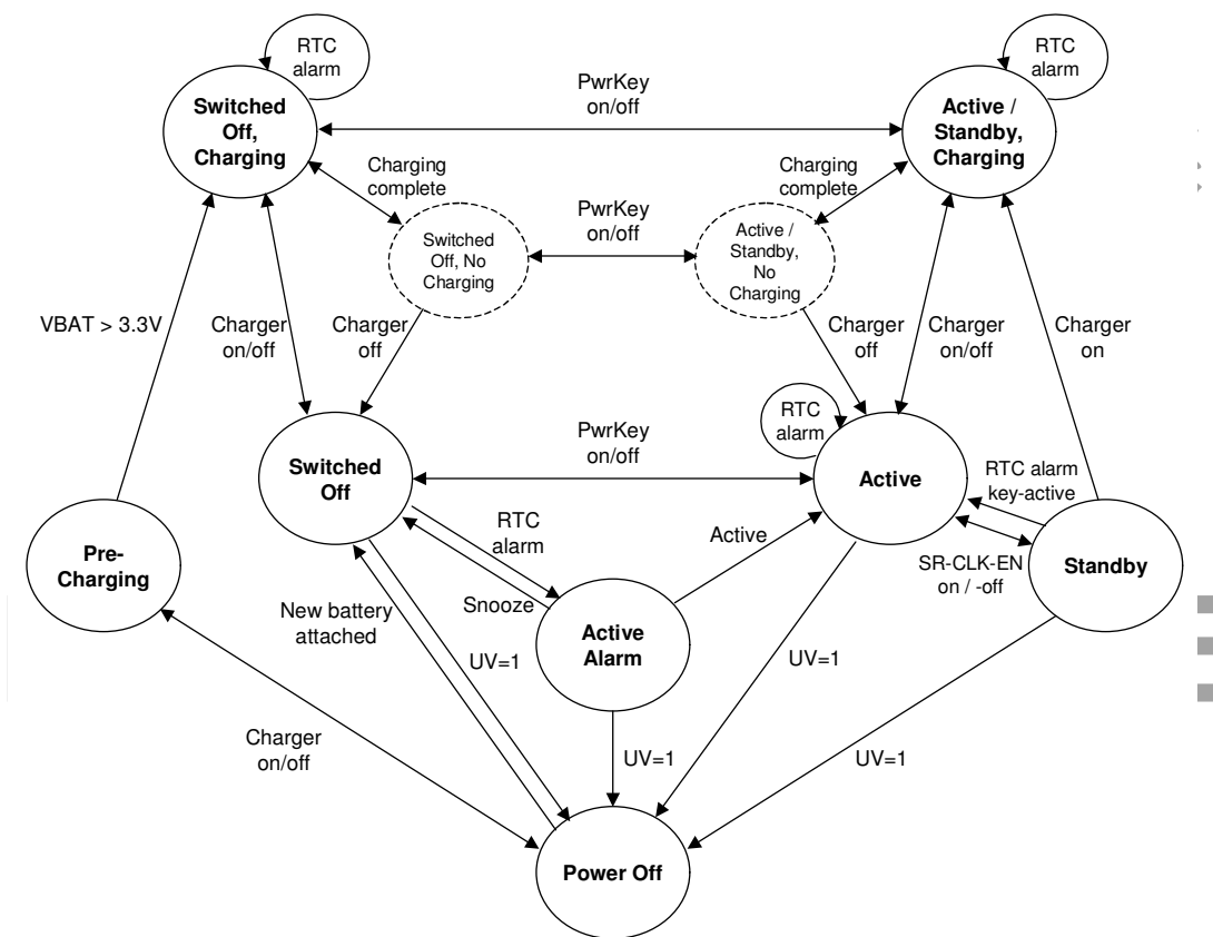
Figure 3: Power Management State Diagram
