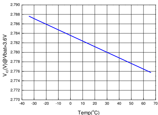
V IO vs. Temp
