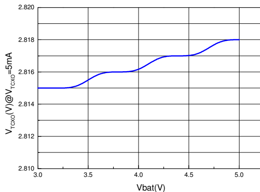
V TCXO vs. V bat
