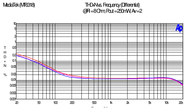
THD+N vs Frequency
