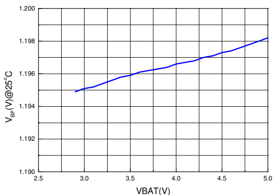
V REF vs. Vbat
