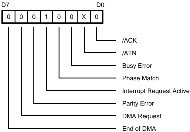
Figure 23. Bus and Status Register
