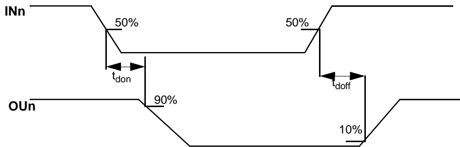
Figure 2. Output delay time
