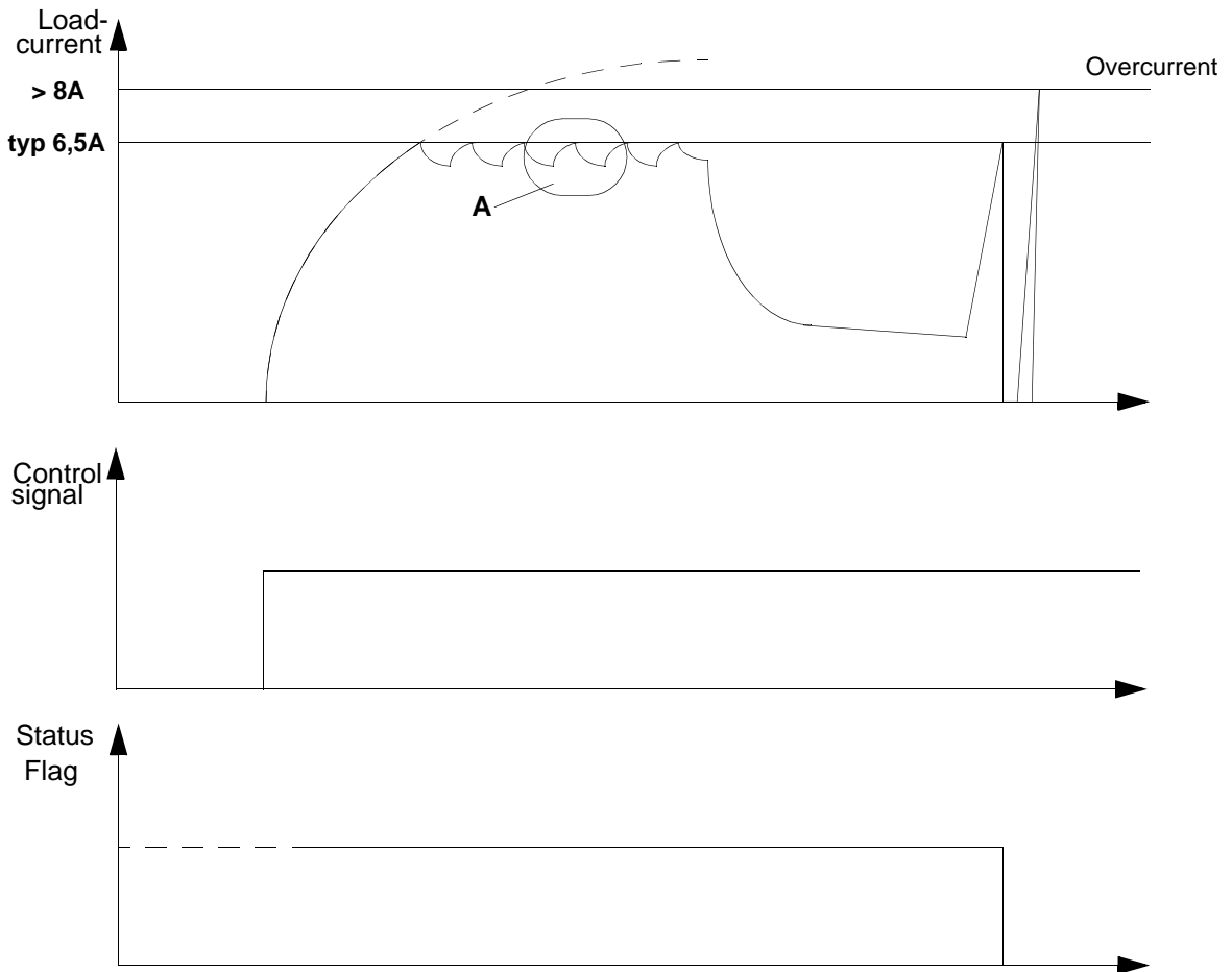
Figure 5. Current Limitation
