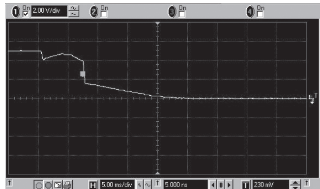
Fall Time (PWM mode): V_{in} = 3.5V ; V_{out} = 5V ; I_{out} = 0.7A
