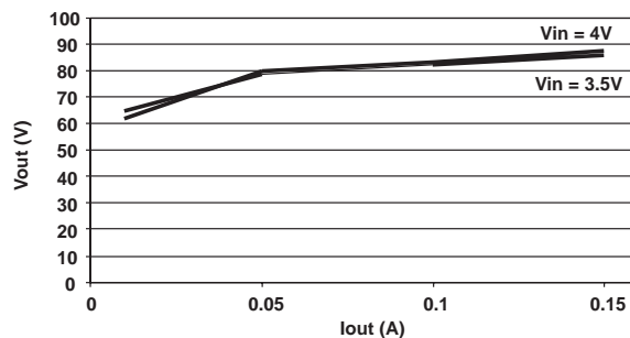
Efficiency Vs. Iout (PSM mode)
