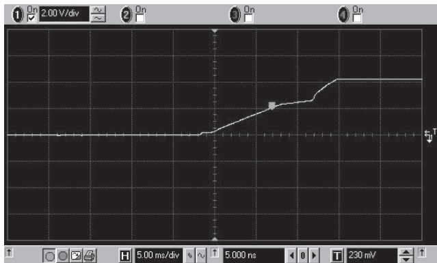
Rise Time (PWM mode): V_{in} = 3.5V ; V_{out} = 5V ; I_{out} = 0.7A
