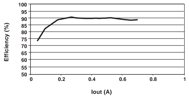
Efficiency Vs. Iout Vin = 3.6V; Vout = 5.0V
