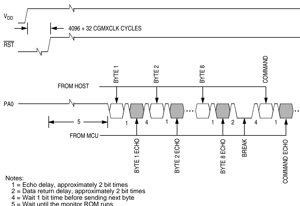
Figure 20-17. Monitor Mode Entry Timing
