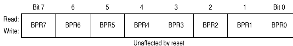
Figure 2-4. FLASH-1 Block Protect Register (FL1BPR)
