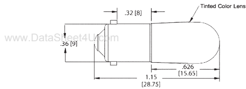
DIALIGHT 586 SERIES SINGLE CHIP BASED LED T-3-1/4 MINIATURE BAYONET (BA9S)
