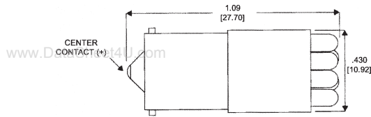
DIALIGHT 585 SERIES CLUSTER BASED LED T-3/4 MINIATURE BAYONET (BA9S)
