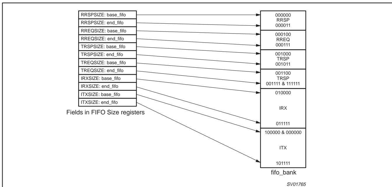
Figure 34. Reset situation of size programmable FIFOs
