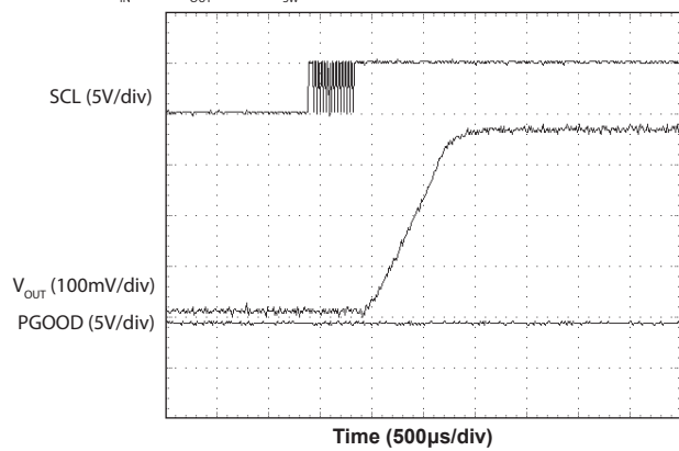
Slew-Up — CCM, 3A Load, EnIntLd=0/1
