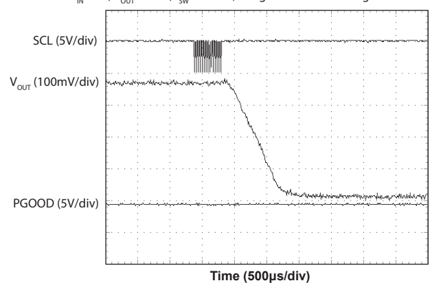
Slew-Down — CCM, 3A Load, EnIntLd=0/1
