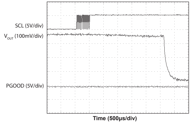
Slew-Down — CCM, No Load, EnIntLd=1
