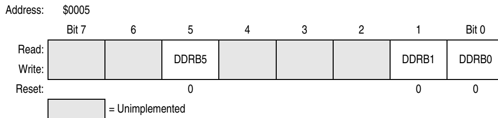
Figure 13-6. Data Direction Register D (DDR)
