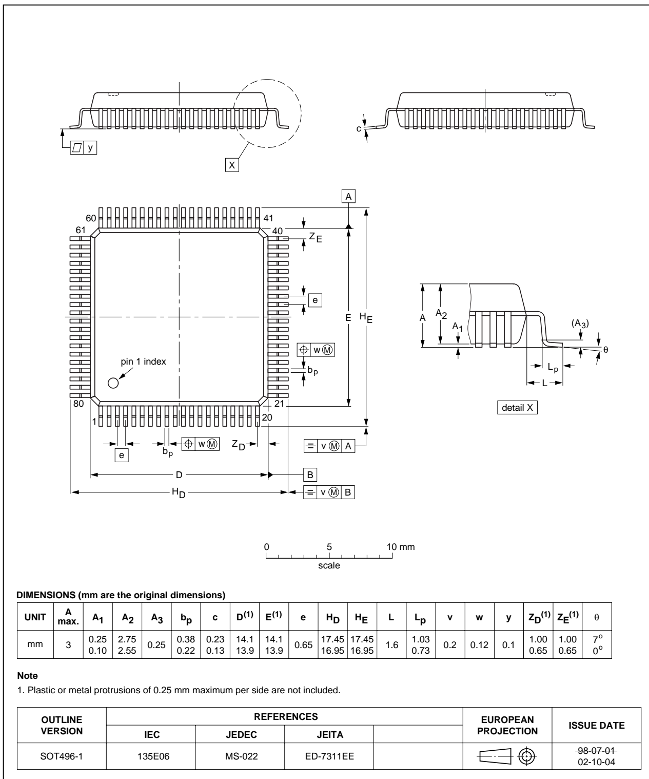
Fig 43. Package outline SOT496-1 (QFP80)
