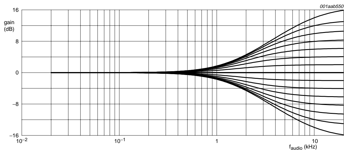
Fig 35. Treble amplitude control characteristics; treble frequency (TRF) = 10 kHz
