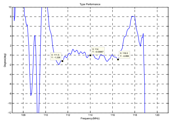
Phase Linearity(f0±2.5MHz)
