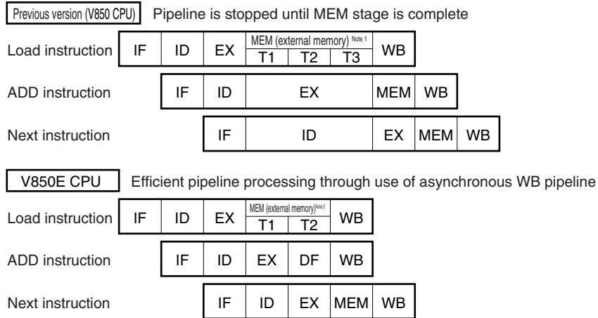
Figure 8-2. Non-Blocking Load/Store
