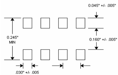
PAD LAYOUT
