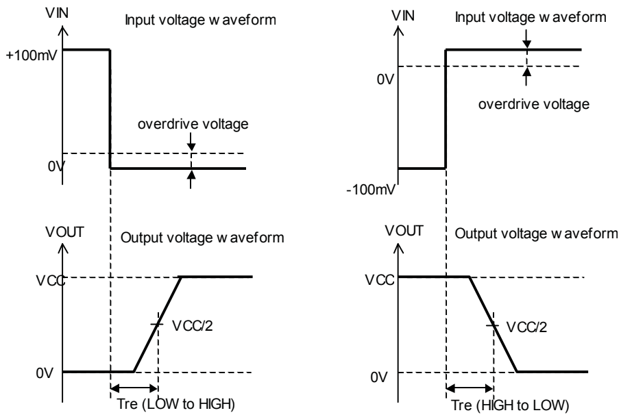
Fig.4 Response Time
