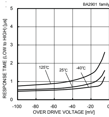
Fig.20 Response Time – Over Drive Voltage (VCC=5[V],VRL=5[V],RL=5.1[kΩ])
