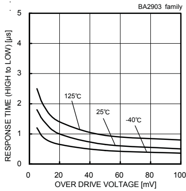
Fig. 22 Response Time – Over Drive Voltage (VCC=5[V],VRL=5[V],RL=5.1[kΩ])
