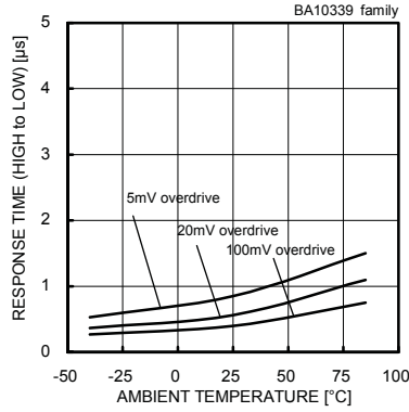
Fig. 20 Response Time HL – Ambient Temperature (VCC=5[V],VRL=5[V],RL=5.1[kΩ])
