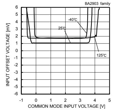
Fig. 18 Input Offset Voltage – Common Mode Input Voltage (VCC=5V)
